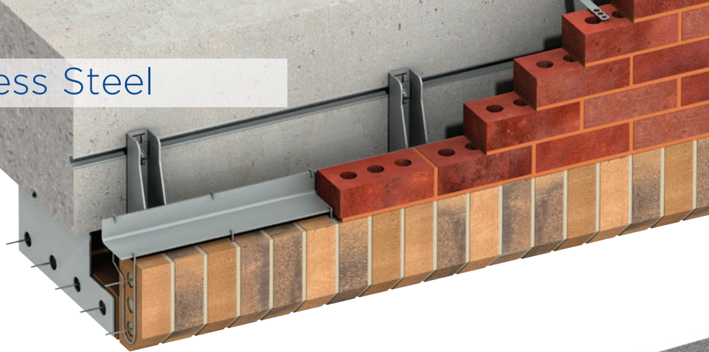
MDC Support System with Stirrups
