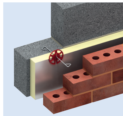
RT2 Wall Tie
