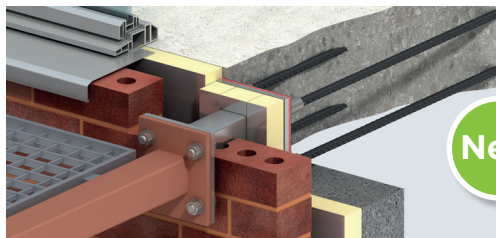
STC/SSTC Steel-to-Concrete Connector Available in either galvanised or stainless steel
