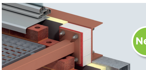
STS/SSTS Steel-to-Steel Connector Available in either galvanised or stainless steel
