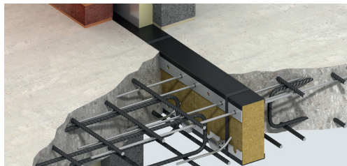
Isotec Concrete-to-Concrete Connector Stainless Steel System
