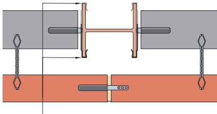
Ancon Hammer-On Ties installed to alternate sides of the column at 225mm vertical centres
