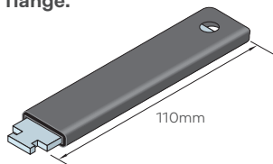
Ancon Hammer-On Tie (Debonded HOS-TIE, pictured above, supplied complete with Hammer-On Section)
