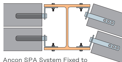
Ancon SPA System Fixed to Steel with Ancon M6 Isolated Set Screws
