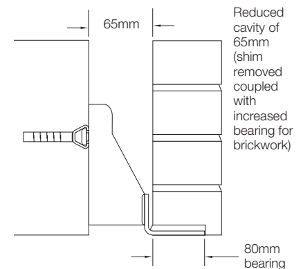
Reduced cavity
