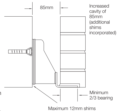
Increased cavity
