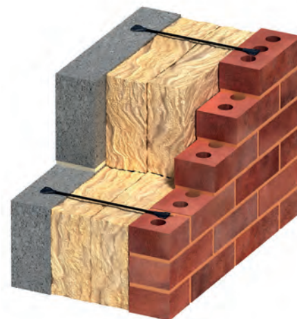
Ancon Teplo-BF Cavity Wall Tie
