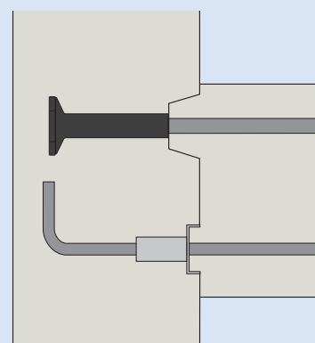
KSN Anchor at top and Ancon Coupler Box on bottom
