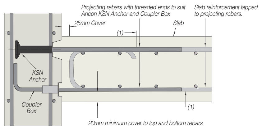
Wall / Slab Section - KSN Anchor at Top / Coupler Box on bottom
