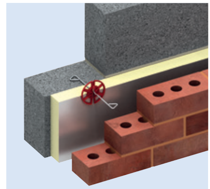
RT2 Wall Tie
