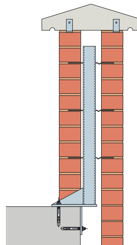
WP1/WP3 Parapet Post Fixed to Top and Face of Concrete
