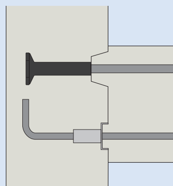
KSN Anchor at top and Ancon Coupler Box on bottom
