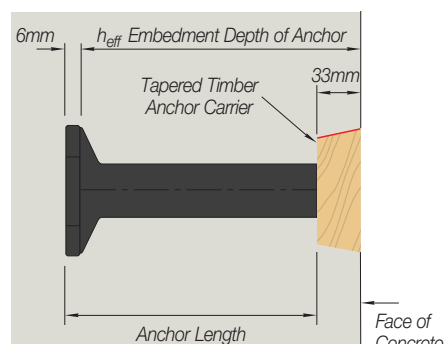
Anchor Embedment Arrangement
