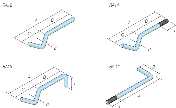
Crook Anchors
