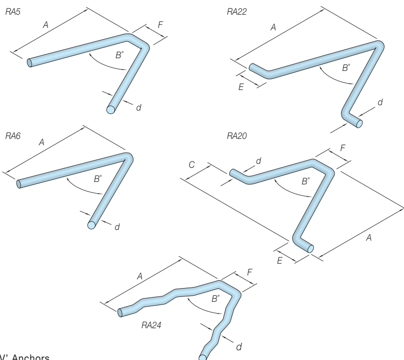
'V' Anchors
