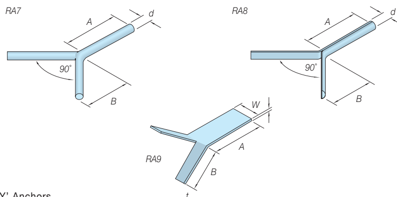
'Y' Anchors
