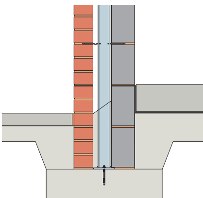
WP3 Windpost Fixed Directly to the Foundations
